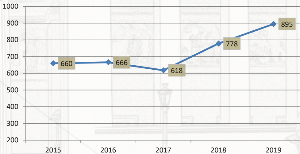
Diagram 3: Number of newly approved SARG programs per year
